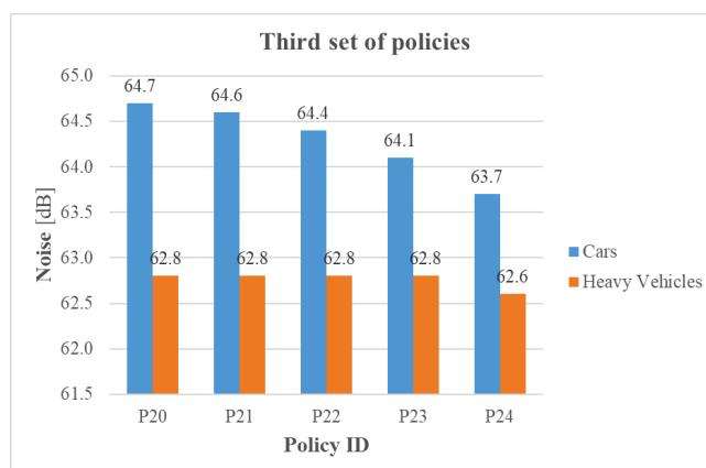
Fig. 8 – Noise values obtained after the application of the third set of policies, in the ascending direction
