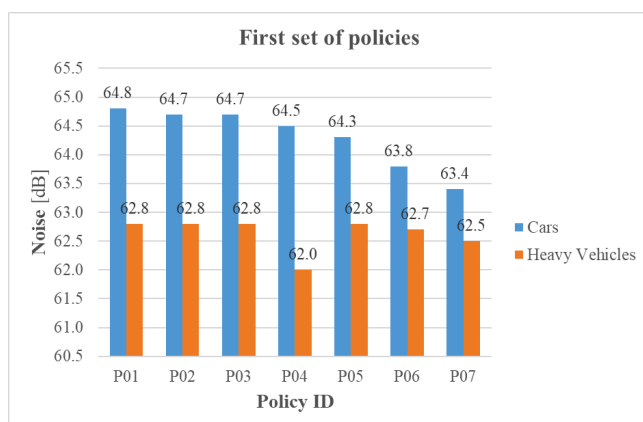
Fig. 6 – Noise values obtained after the application of the first set of policies, in the ascending direction
