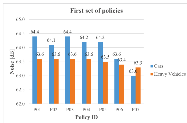
Fig. 9 – Noise values obtained after the application of the first set of policies, in the descending direction
