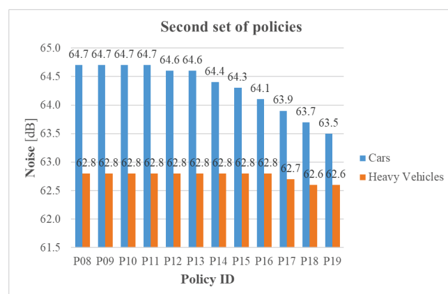
Fig. 7 – Noise values obtained after the application of the second set of policies, in the ascending direction
