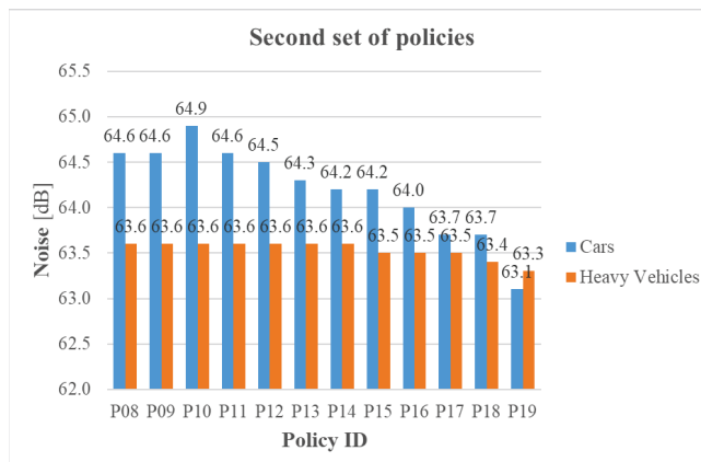
Fig. 10 – Noise values obtained after the application of the second set of policies, in the descending direction
